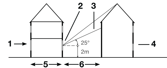
1. Additional light from rear 2. raise window head height 3. Daylight obstructed 4. Obstructing building 5. Shallow plan 6. Less than 10m
