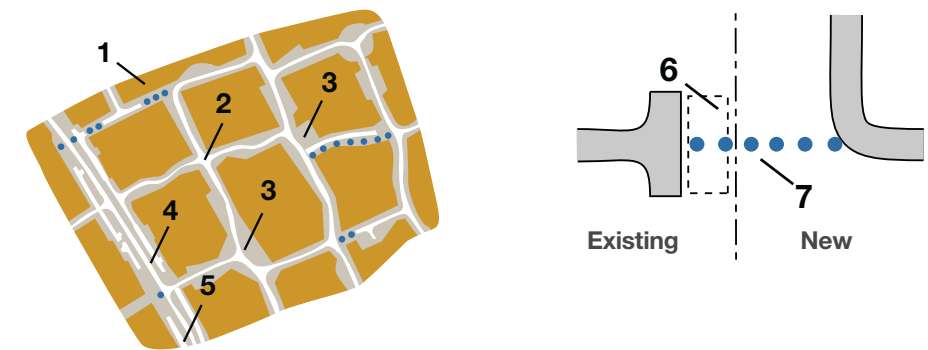
1. Pedestrian/cycle street linking parts of road network 2. Crossroads possible where one branch serves few dwellings 3. Nodal point 4. Frontage to major road reserved by private drives 5. Pedestrian/cycle link across major road 6. Ransom strip prohibits vehicle access 7. Pedestrian/cycle link between new and existing
