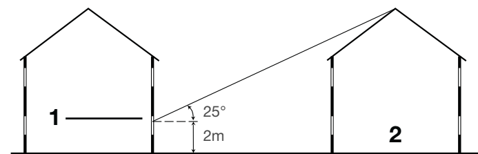
1. Reference line for daylight calculation 2. Obstructing building
