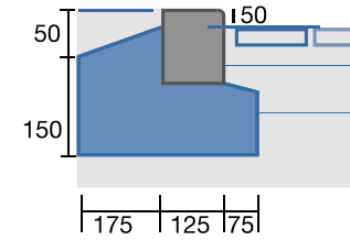
Edge detail with paviors
