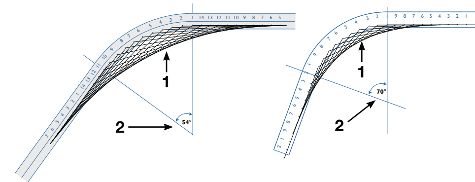
1. Forward visibility curve 2. deflection angle
