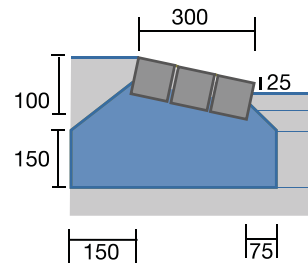
Suggested kerb treatment on Type 5 roads
