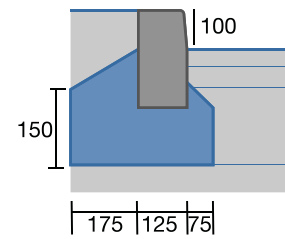
Upstand Kerb to road Types 1, 2 and 3
