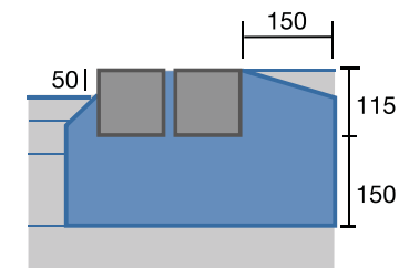
Granite sett kerb
