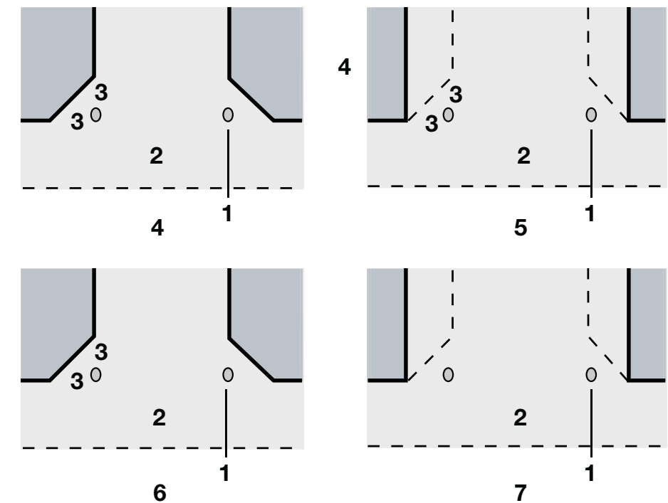
1. Bollards 2. Footway 3. 1.5 pedestrian/vehicle visibility dispaly 4. Splays cut out of buildings or walls 5. Entrance widened by 1.5m on each side 6. Buildings or walls set back 1.5m behind back edge of footway 7. Buildings set back and entrance widened by less than 1.5m each
