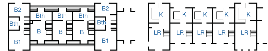
First floor plans (combination of 1&2 bed terrace houses)
