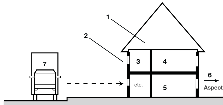
1. Continuous barrier block 2. Small acoustically double glazed windows 3. Bathroom 4. Bedrooms 5. Living rooms 6. Interior of site protected from noise by barrier block 7. Noise source
