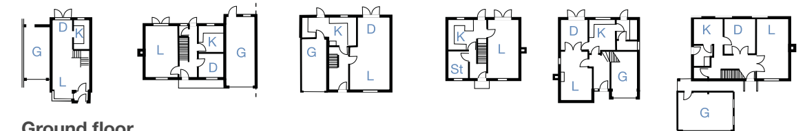
Ground floor
