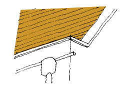
Correct Parapetted gable and eaves
