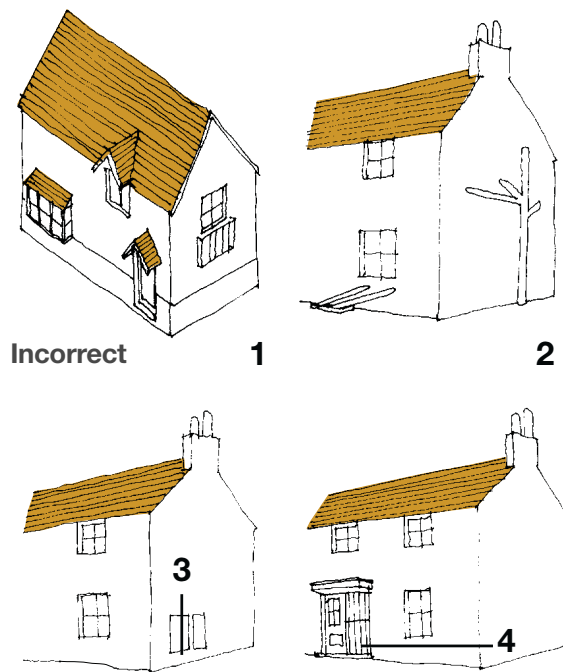
Acceptable positions for meters and service intakes
